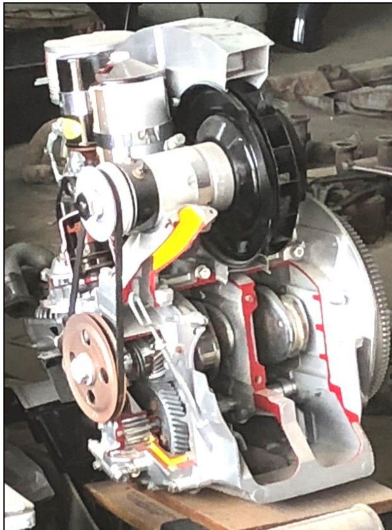
Cutaway 356 engine picture from Adam Wright
